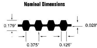
0.375" Pitch (DL) Light Duty Dual Synchronous Timing Belts
